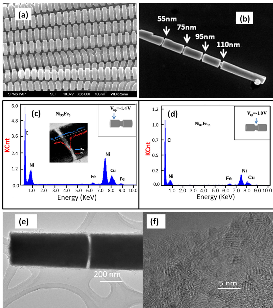
FIG. 3. (a) SEM image of constricted \text{Ni}_{95}\text{Fe}_5 ( l = 125 nm, \varnothing = 350 nm)/ \text{Ni}_{87}\text{Fe}_{13} ( l = 50 nm, \varnothing = 250 nm) nanowires. (b) A free standing individual strand of constricted \text{Ni}_{95}\text{Fe}_5/\text{Ni}_{87}\text{Fe}_{13} nanowire with different dimension of constriction. (c), (d) EDX measurements of the \text{Ni}_x\text{Fe}_{1-x} nanowire deposited at applied potentials of -1.4 V and -1.0 V. The composition is determined to be \text{Ni}_{95}\text{Fe}_5 and \text{Ni}_{87}\text{Fe}_{13} . Inset shows EDX elemental line scanning of Ni and Fe elements (Ni red, Fe blue) along the multilayered \text{Ni}_{95}\text{Fe}_5 and \text{Ni}_{87}\text{Fe}_{13} nanowires. (e) TEM image of a constricted \text{Ni}_{95}\text{Fe}_5/\text{Ni}_{87}\text{Fe}_{13} nanowire. (f) Surface analysis morphology at the tip of the nanowire. The results indicate that the nanowire is polycrystalline with an alternate segment of \text{Ni}_{95}\text{Fe}_5 and \text{Ni}_{87}\text{Fe}_{13} .
