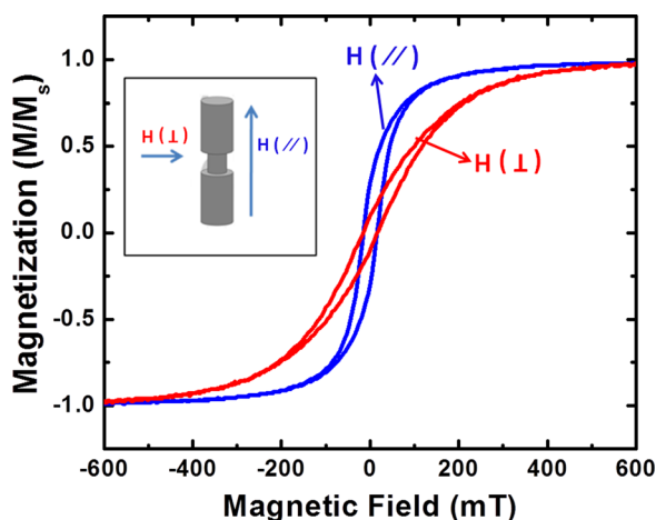
FIG. 4. Hysteresis loop measurements of the constricted \text{Ni}_{95}\text{Fe}_5/\text{Ni}_{87}\text{Fe}_{13} nanowires with a magnetic field applied parallel, H (//) and perpendicular, H (\perp) to the nanowire axis.
